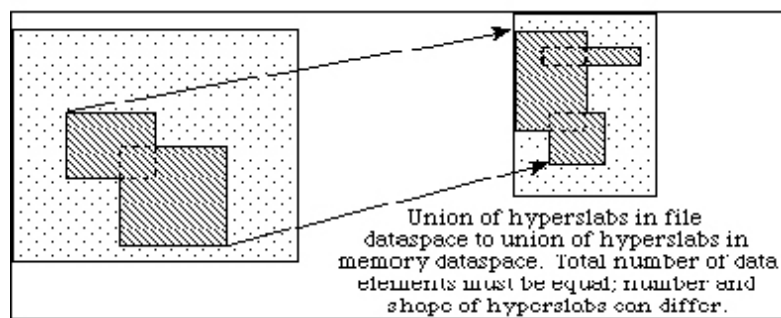
Figure 6. Build complex regions with hyperslab unions
