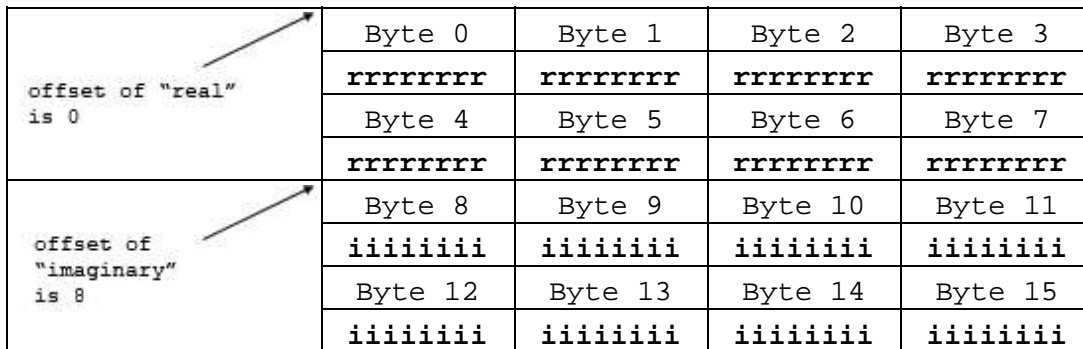
Figure 11. Layout of a compound datatype
