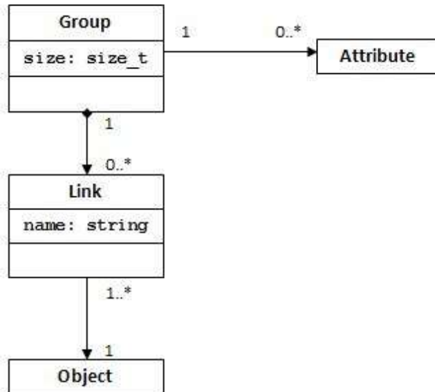
Figure 4. Abstract model of the HDF5 group object
