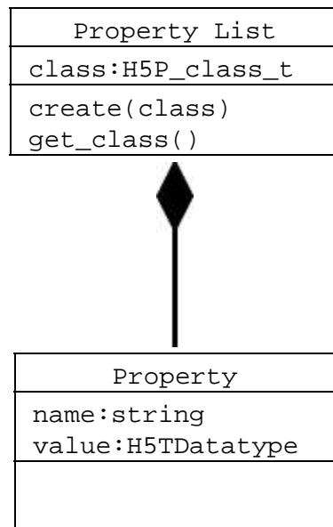
Figure 11. The property list
