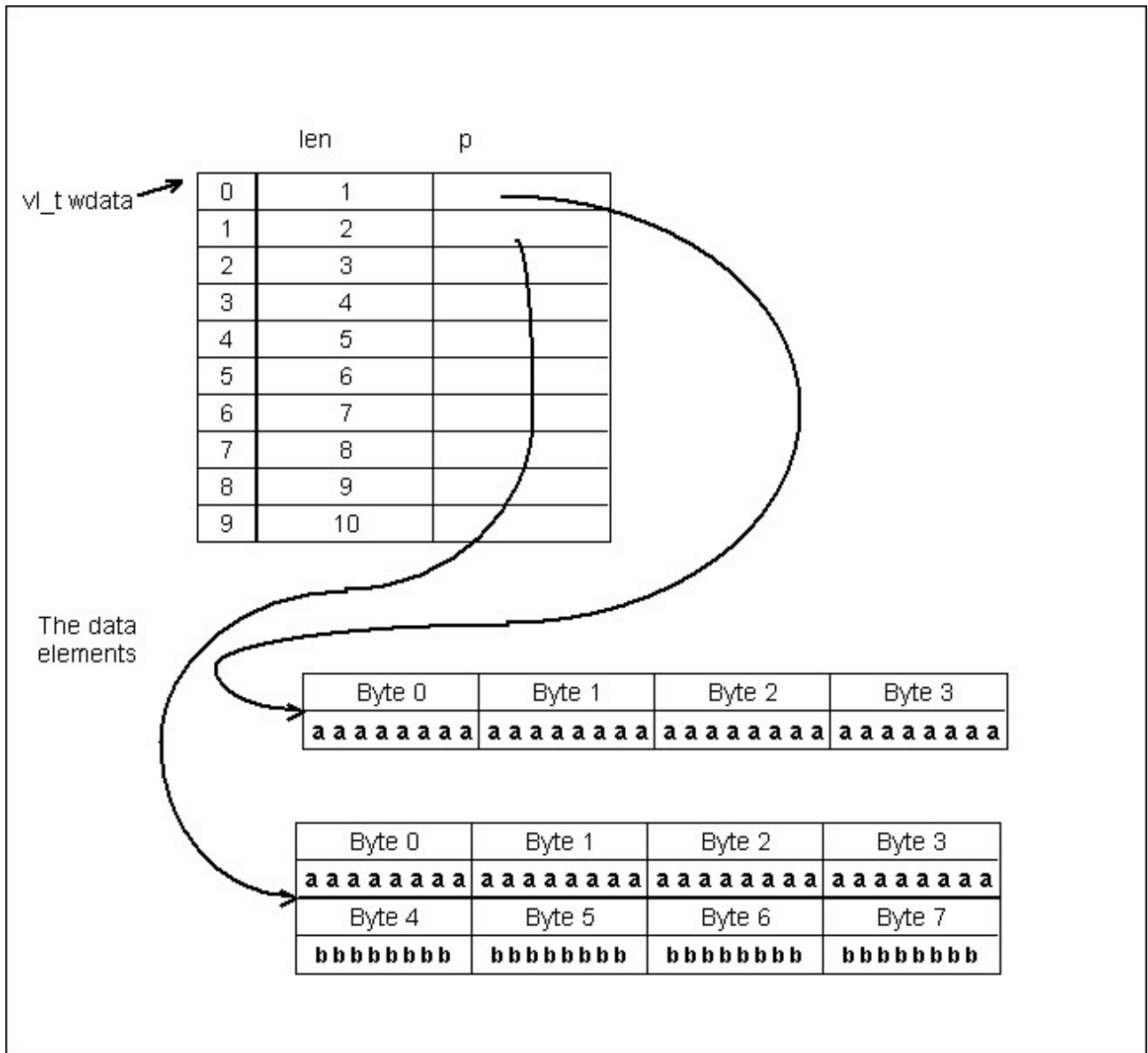
Figure 16. Memory layout of a VL datatype
