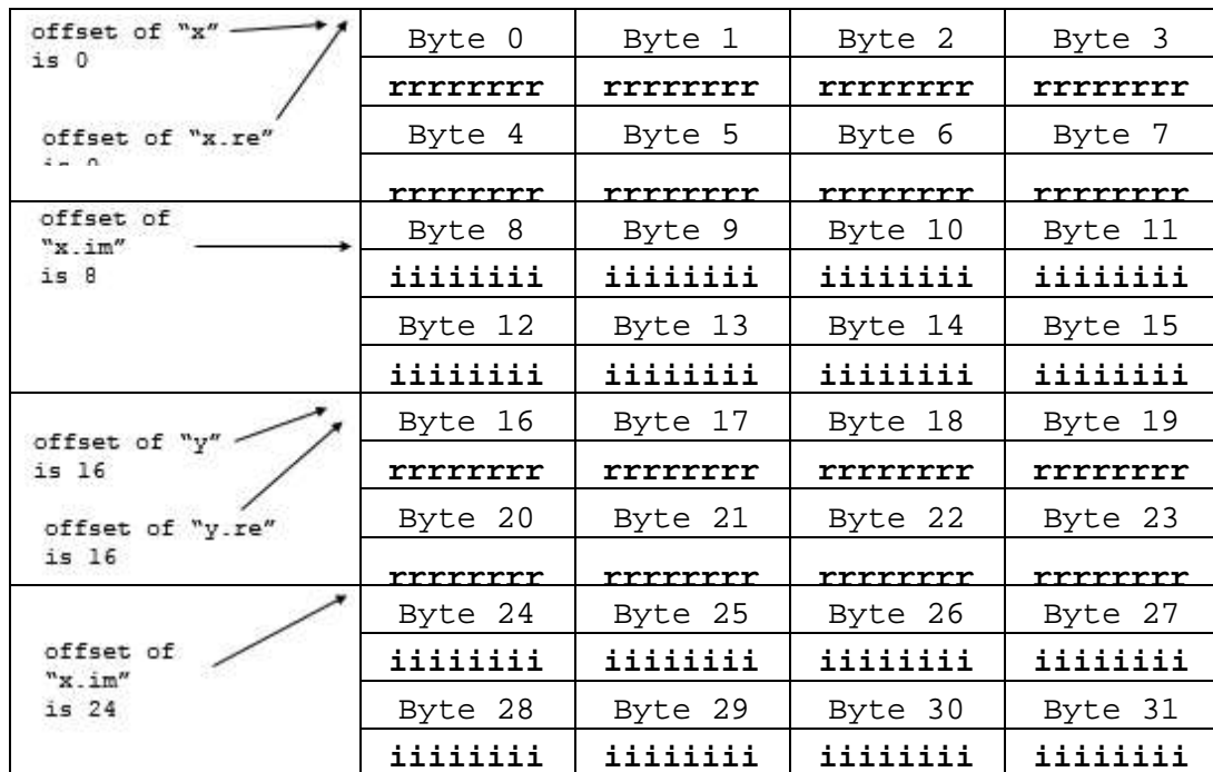
Figure 12. Layout of a compound datatype nested within a compound datatype
