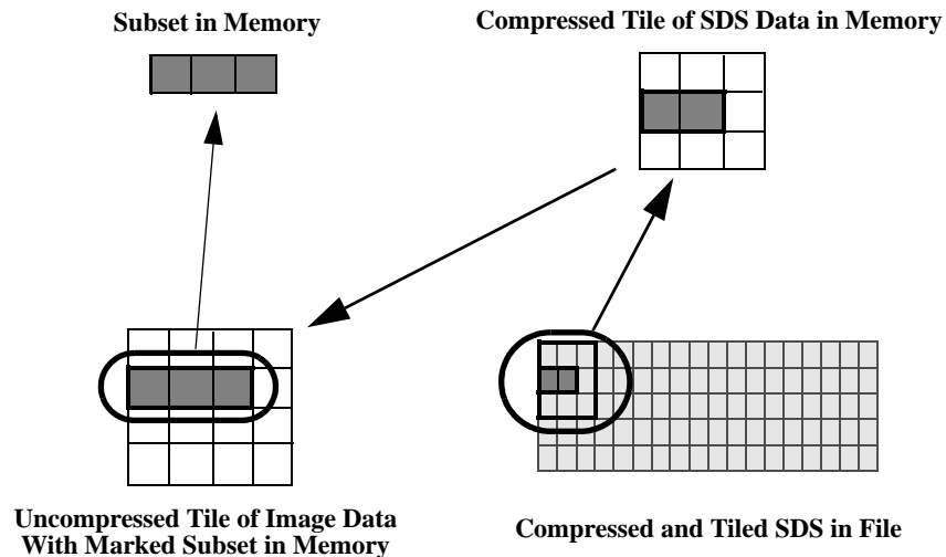
Extracting a Subset from a Compressed and Tiled SDS
