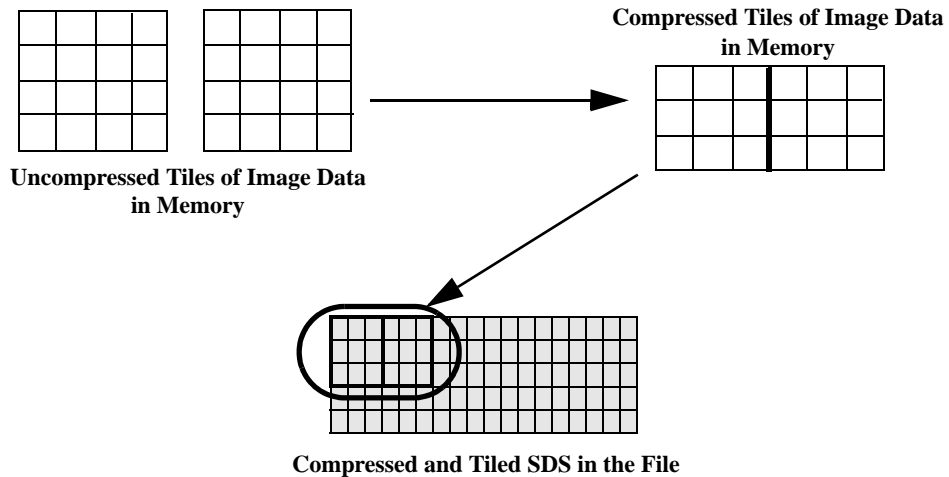
Compressing and Writing Chunks of Data to a Compressed and Tiled SDS
