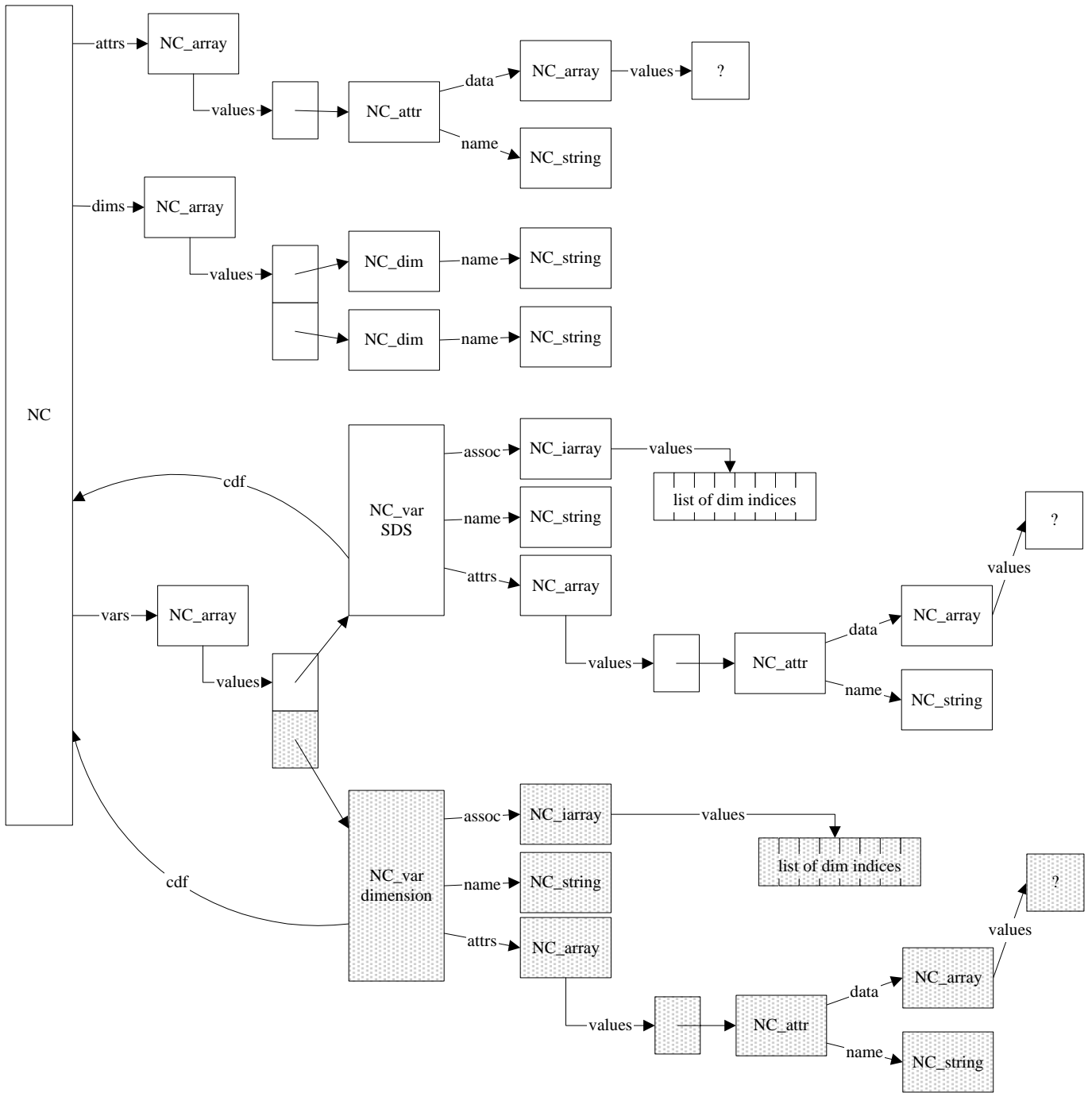
SD collection contents in memory after adding a dimension attribute
