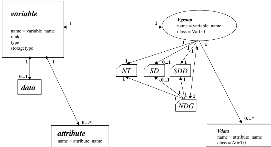
Model-to-File Mapping -- variable, data, and attribute
