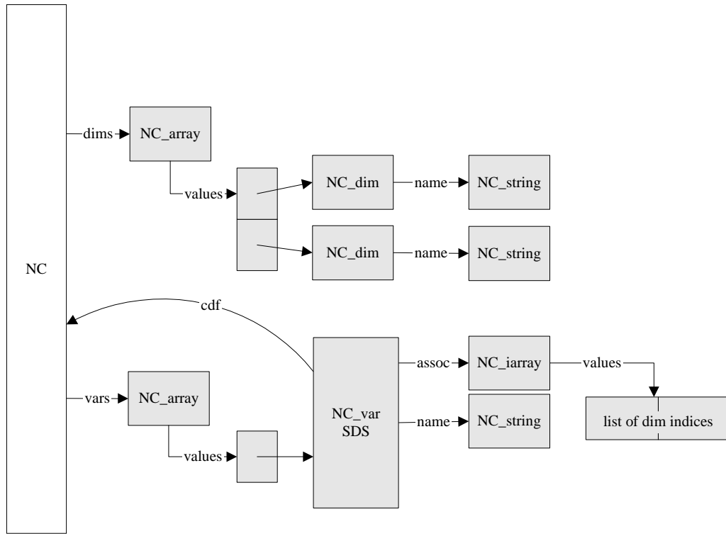
SD collection contents in memory after a 2-dimensional SDS is created
