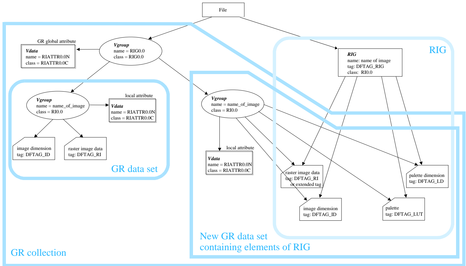
File of Figure 8l after GR API has been used to add an attribute to the RIG image
