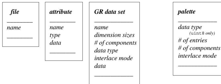
GR Data model objects
