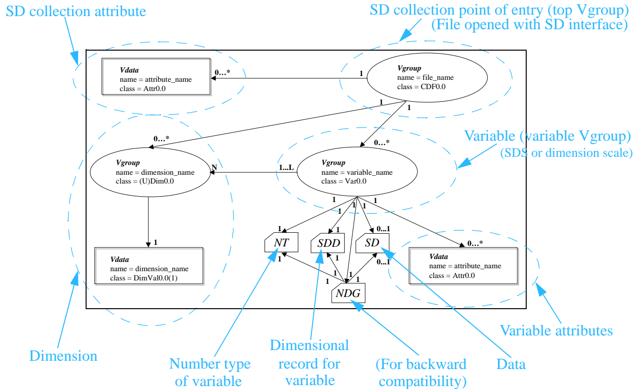
Developer's view of the SD model (Figure 7h) and the corresponding elements of the HDF file structure (Figure 7o)
