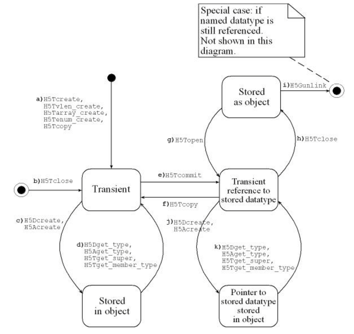
Figure 6-23. Life cycle of a datatype
