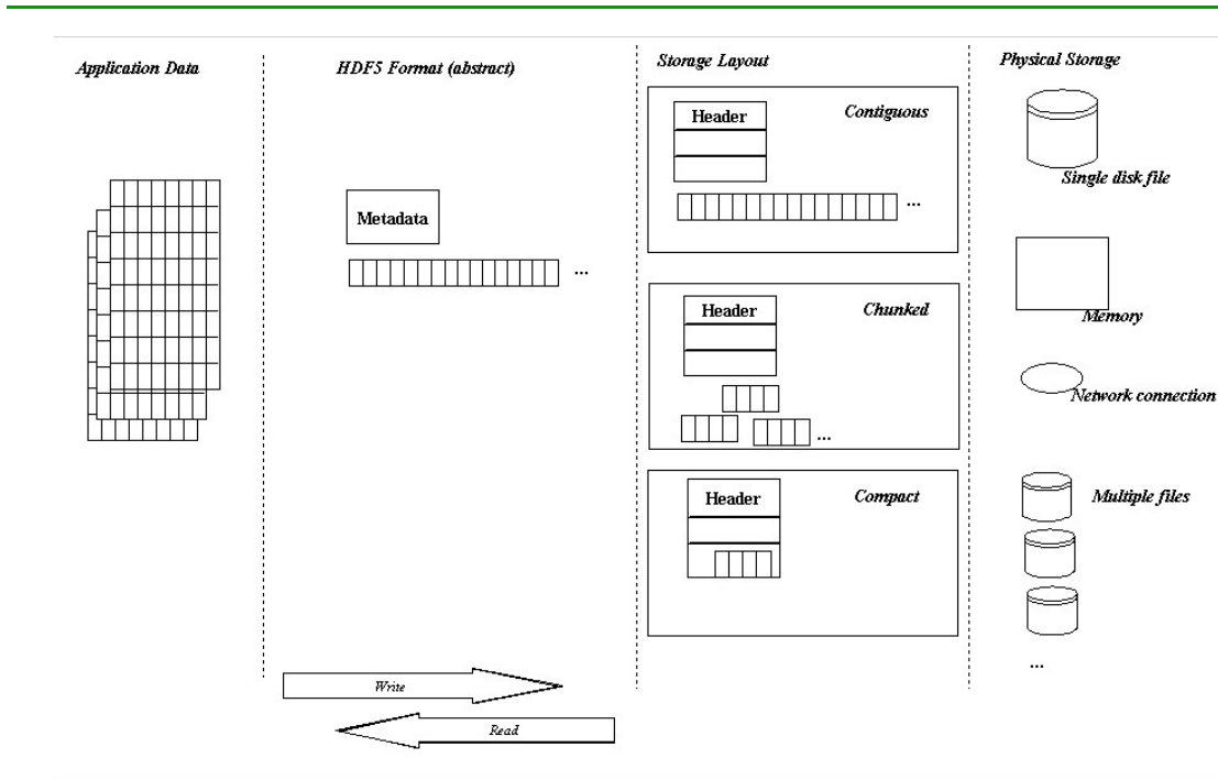
Figure 5-4. Data layouts in an application
