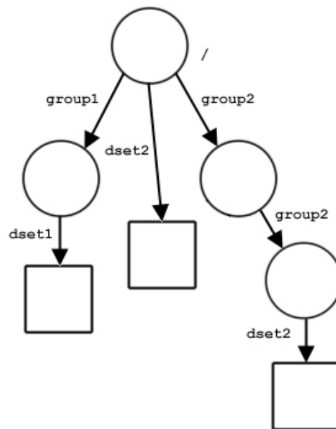
Figure 1-17. Another HDF5 file structure with groups and datasets
