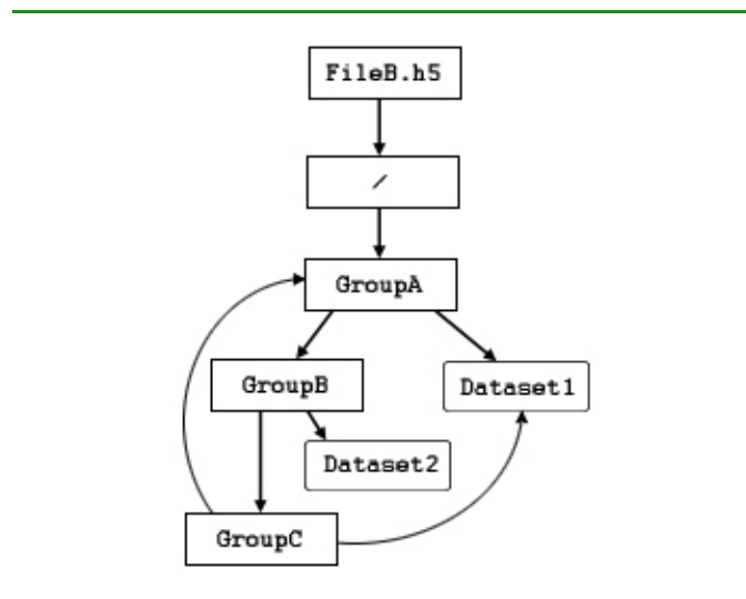
Figure 4-8. A file with a circular reference
