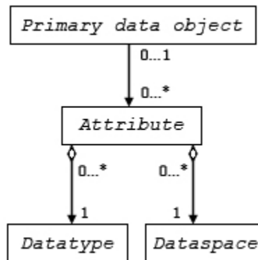
Figure 8-1. The UML model for an HDF5 attribute
