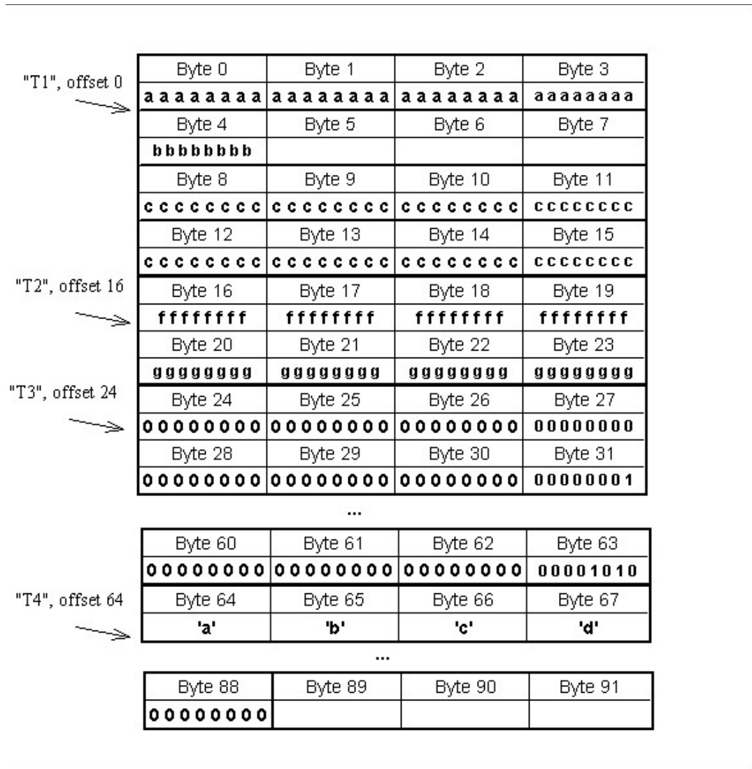
Figure 6-21. The storage layout of the combined four members
