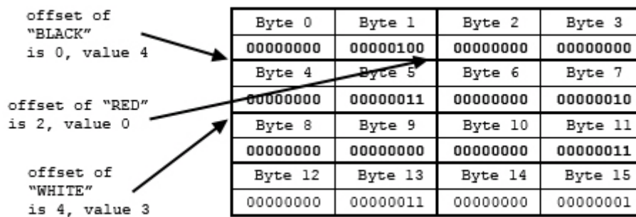
Figure 6-17. Storing an enum array
