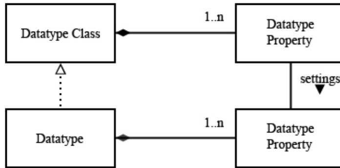
Figure 6-2. The datatype model
