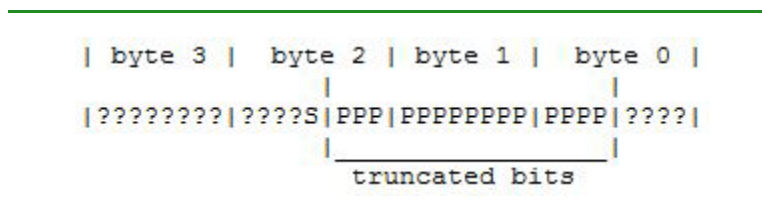
Figure 5-14. Passed to the n-bit filter
