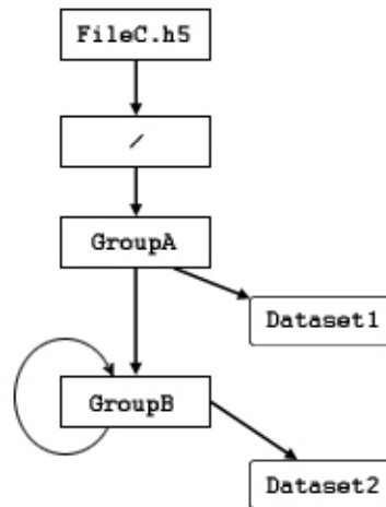
Figure 4-3. A file with one group as a member of itself
