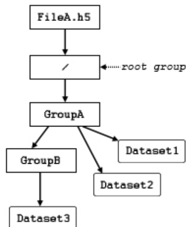
Figure 4-1. A file with a strictly hierarchical group structure
