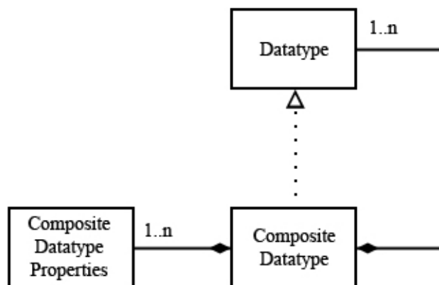
Figure 6-3. Composite datatypes
