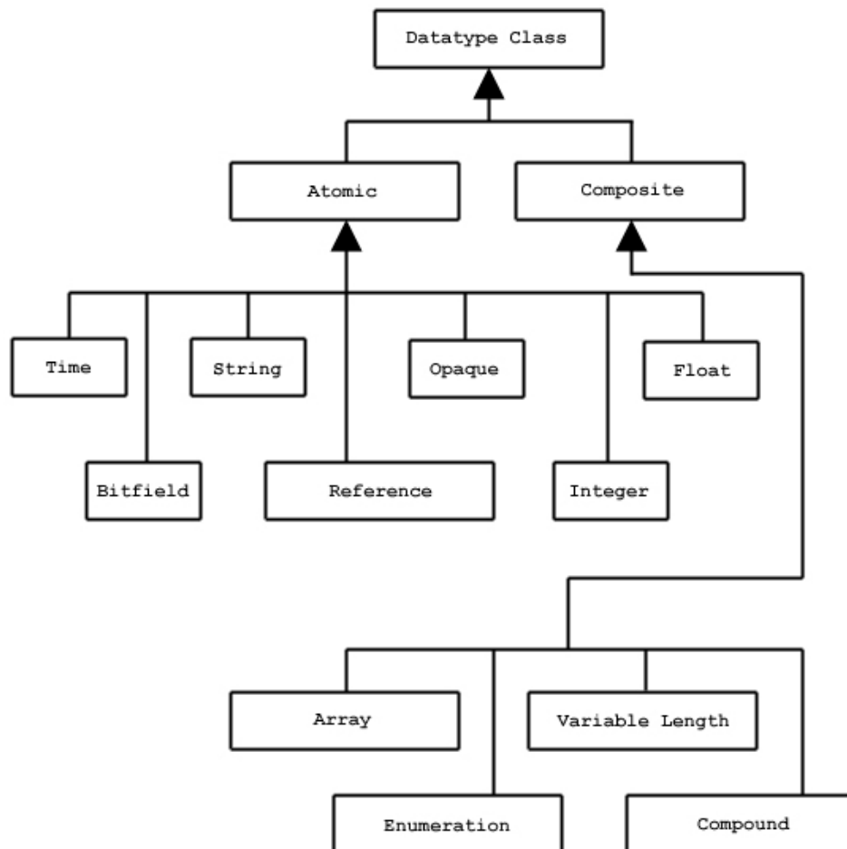
Figure 6-4. Datatype classes
