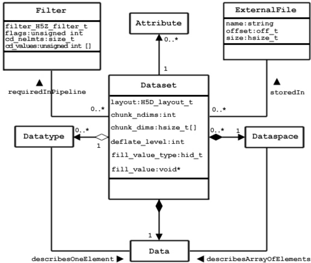
Figure 1-7. The dataset
