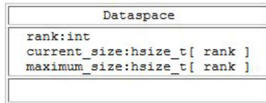
Figure 1-8. The dataspace
