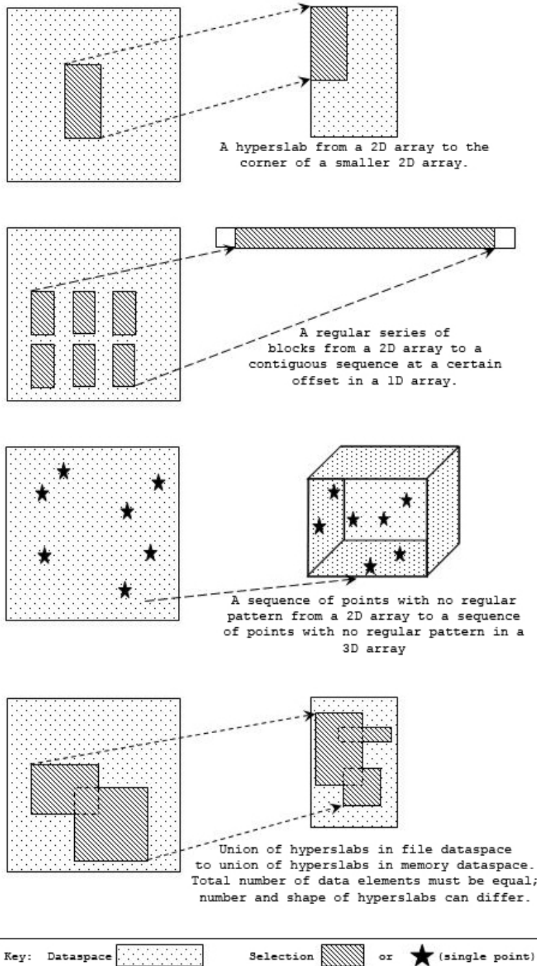
Figure 2-1. Dataset selections
