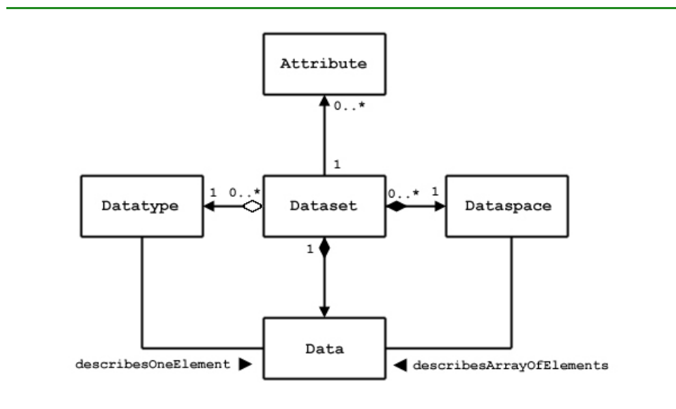
Figure 5-1. Application view of a dataset
