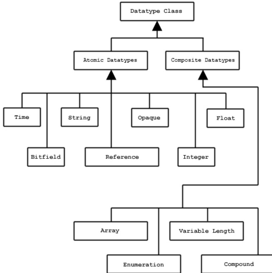
Figure 1-9. Datatype classifications
