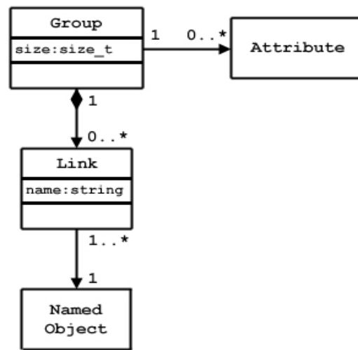
Figure 1-5. Group membership via link objects
