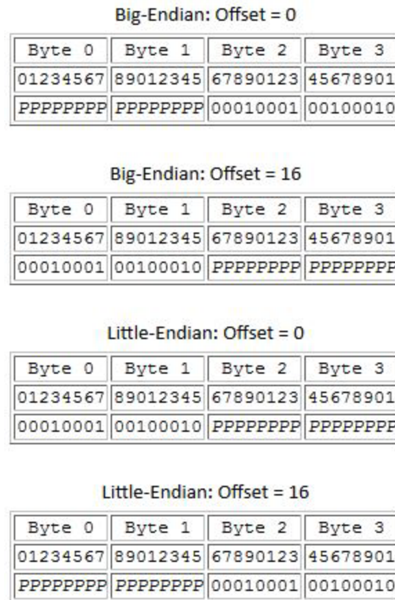
Figure 6-7. Memory Layout for a 32-bit unsigned integer
